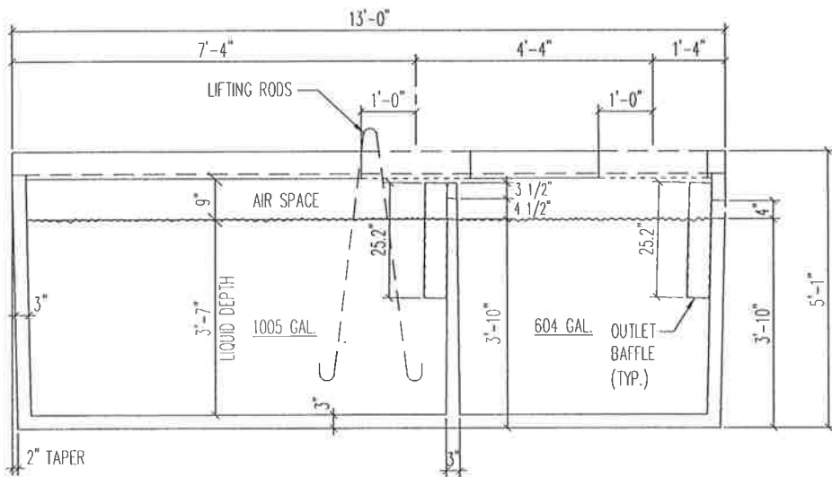
SECTION A-A 1/2" = 1'-0"
